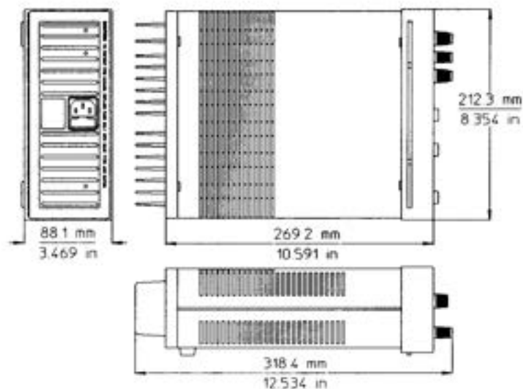
Figure 1: OUTLINE DIAGRAM
